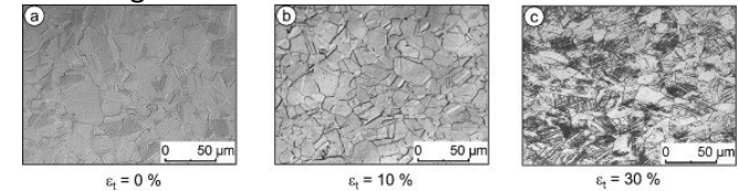
Light micrographs related to stress-strain and magnetic fraction-strain curves of AISI 304
