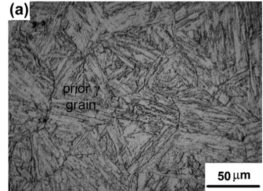
X12Cr13 – OM microstructure
